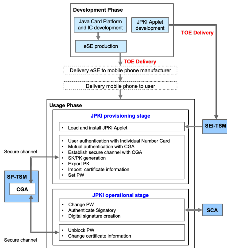
Figure 1-2 TOE lifecycle
