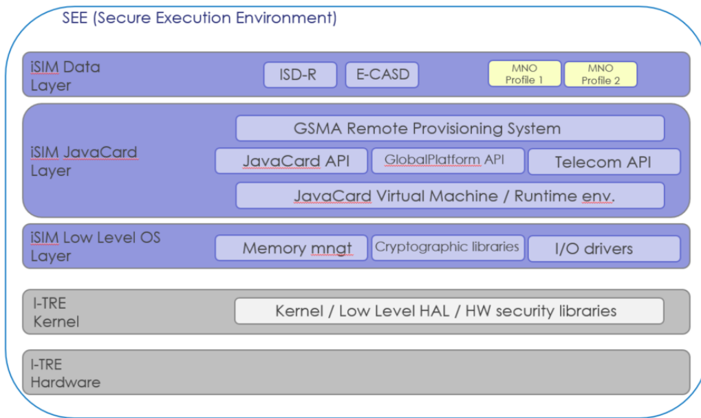
Figure 2 – iSIM v4.0 overview
