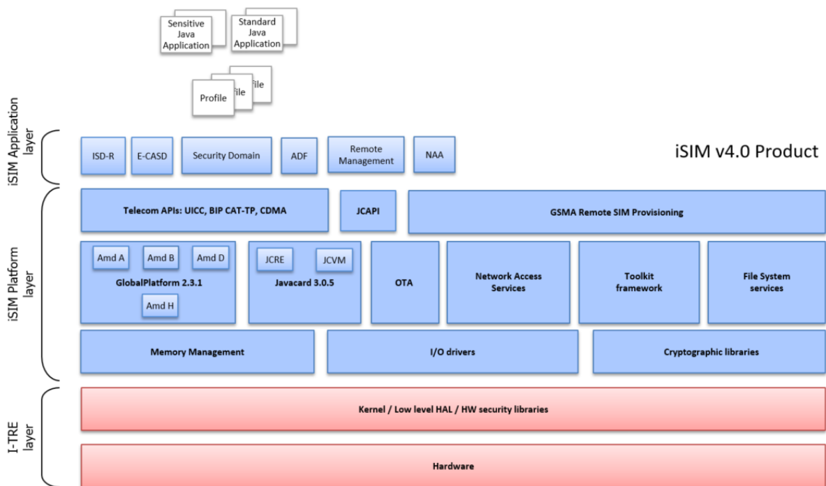
Figure 3 – iSIM v4.0 architecture
