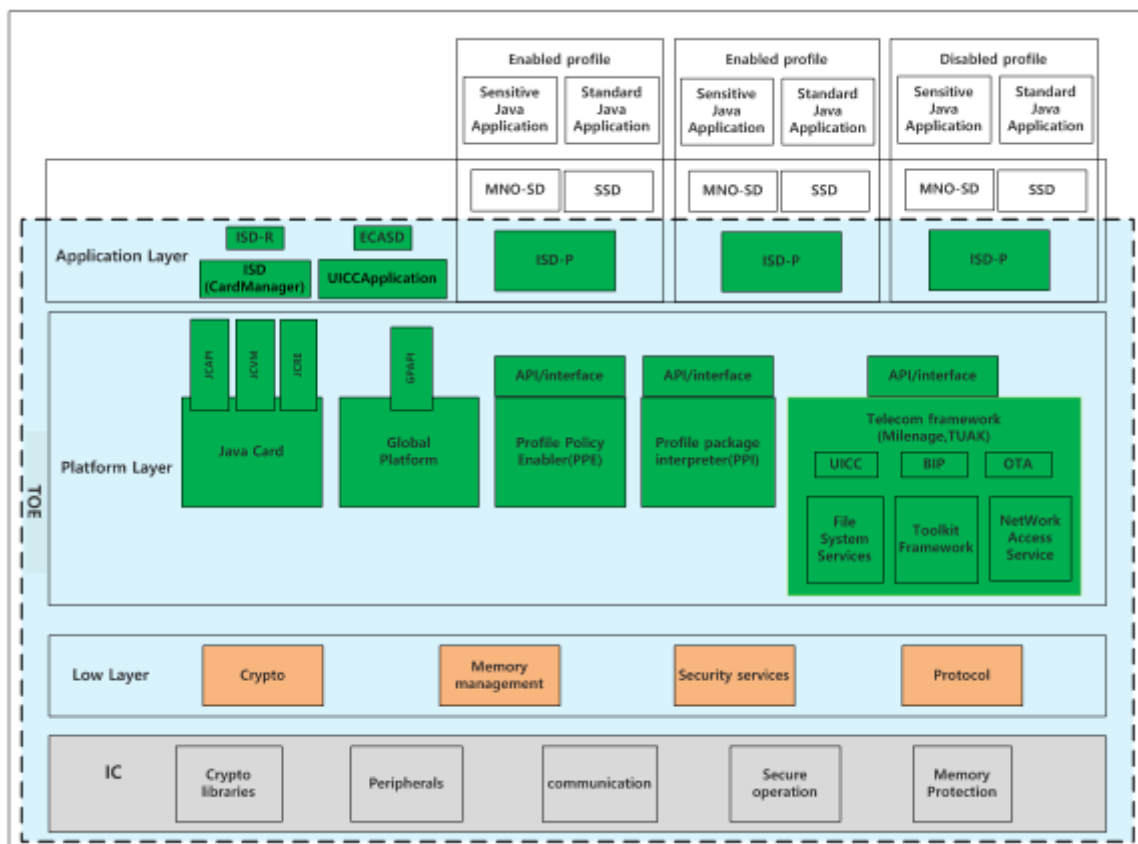
Figure 1 TOE Architecture
