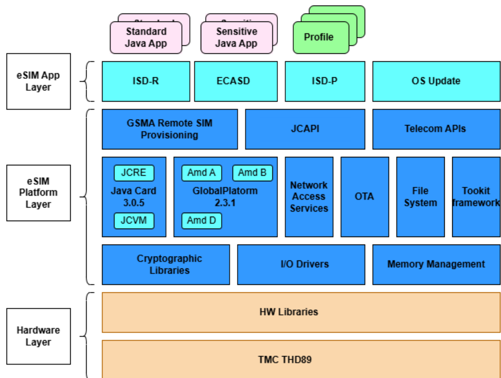
Figure 2 – TMC-E92-B eUICC RSP V1.1 architecture overview
