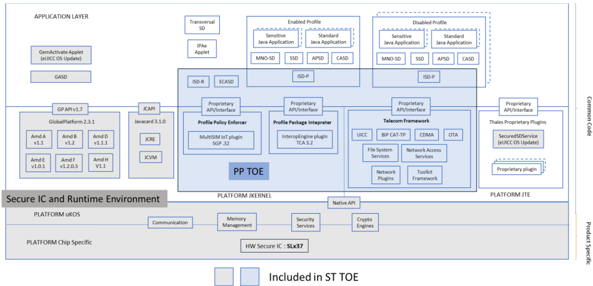
Figure 2 - MSM IOT 9.3.1 v2.0 Platform architecture
