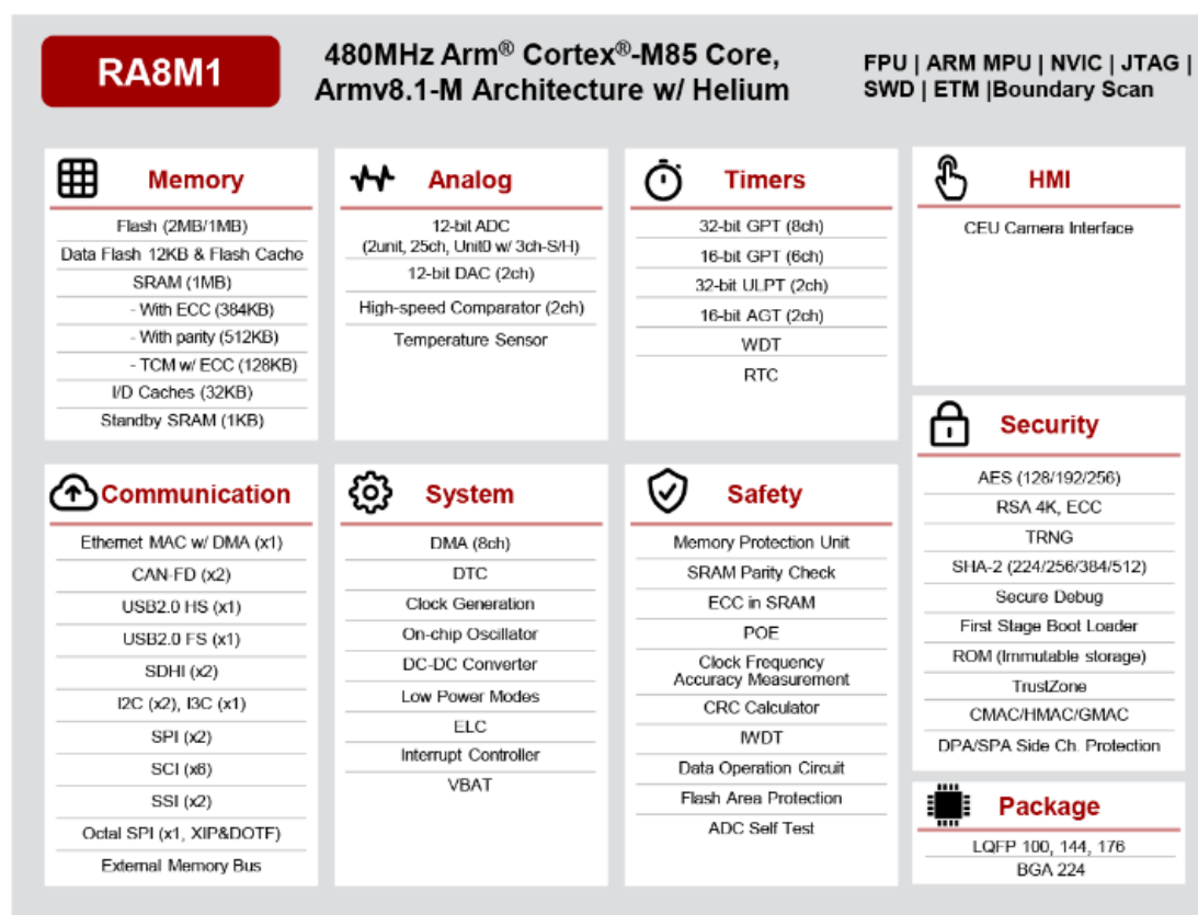
Figure 1-1 RA8M1 MCU Group Block Diagram
