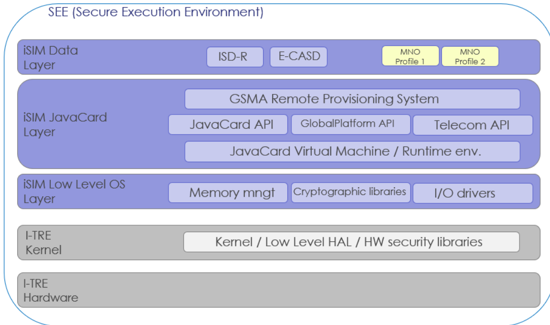
Figure 2 – iSIM for SM8650 overview
