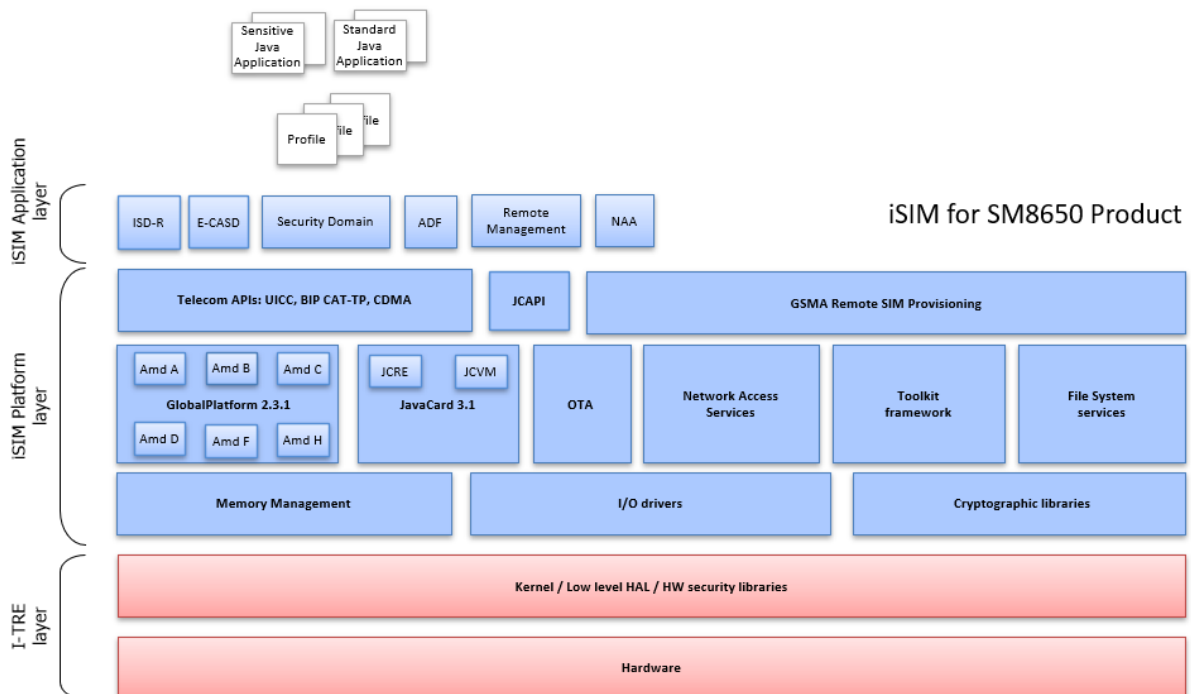
Figure 3 – iSIM for SM8650 architecture
