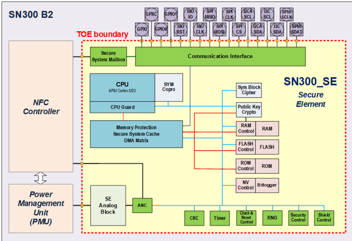
Figure 1 TOE Architecture
